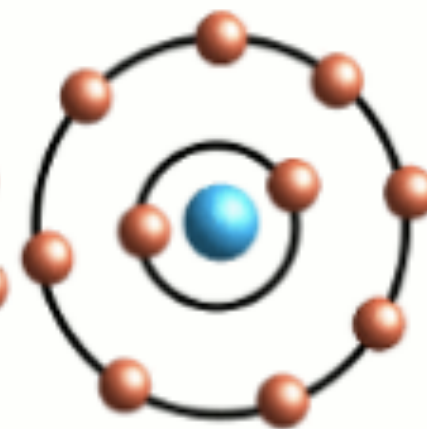
Neon
