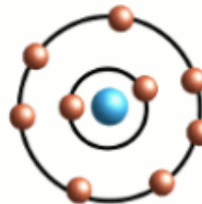
Fluor
