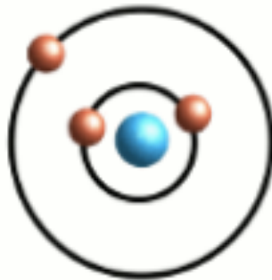
Lithium
