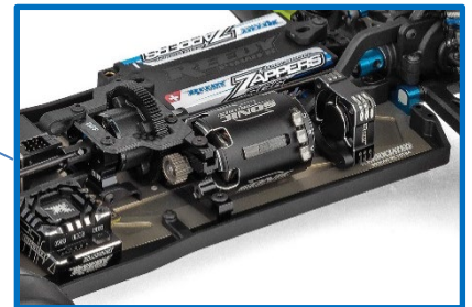
V2 Side Rails to Account for Wide Tongue Chassis
