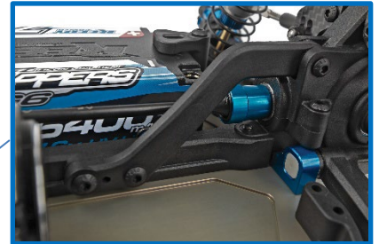
Chassis Bracing: Fine tune chassis flex characteristics with upper and lower chassis bracing front and rear
