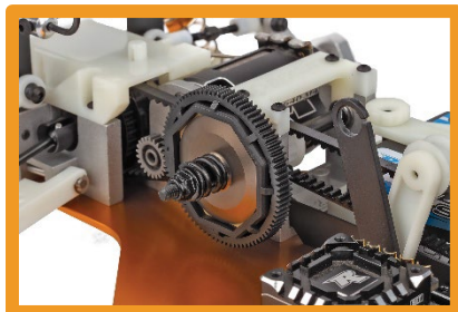
Slipper Clutch
