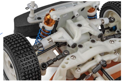
New fully adjustable front upper arms
