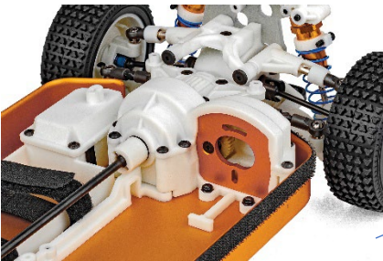
Hardened steel driveshafts and axles
