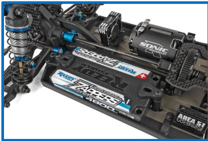
102mm Center CVA Dog Bone Included
