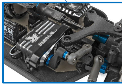
V2 Steering Posts and Bellcranks to Reduce Vertical Movement in the Steering Rack
