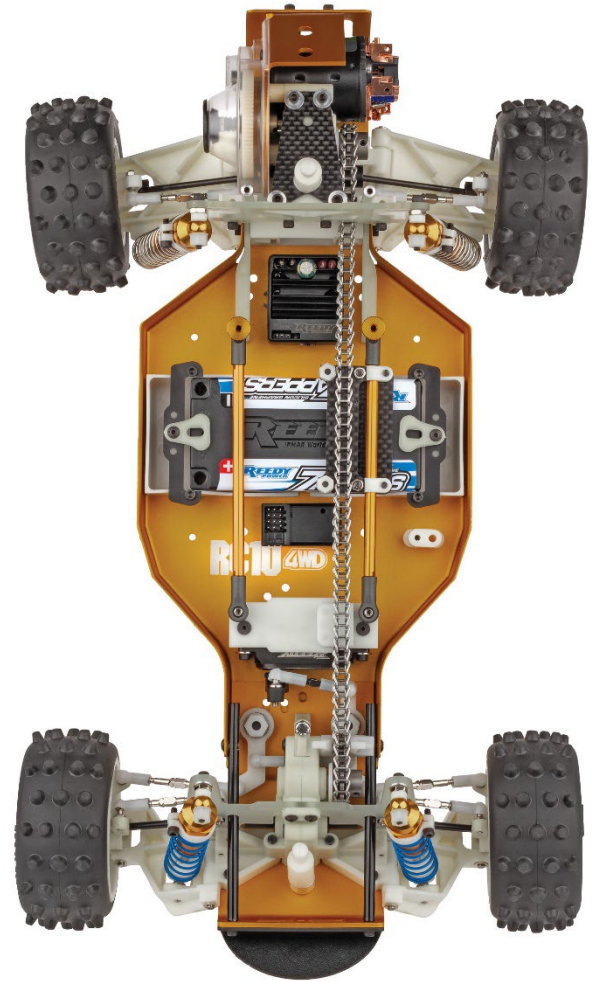
Short front arm geometry and fluid filled anodized aluminum coil over shocks
