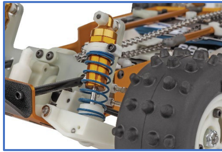
Short front arm geometry and fluid filled anodized aluminum coil over shocks
