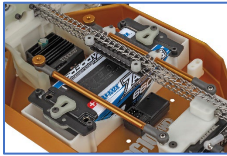
New carbon fiber chain separator system
