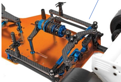
Integrated droop posts for adjusting droop without disassembly
