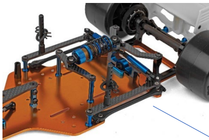
FOX® Genuine Kashima Coat center shock for minimal friction and extended wear
