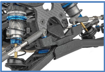
NEW -2mm Front Ballstud Mount included along with updated Top Plate and Standard Ballstud Mount
