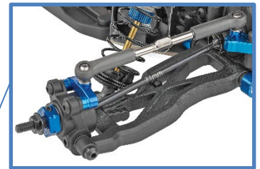
81mm Rear Suspension Arms and 71mm CVA Bones
