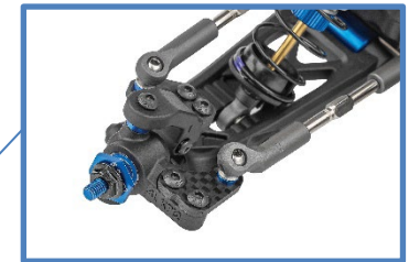
NEW Steering and Caster Block Assembly simplifies assembly and reduces weight without sacrificing tunability
