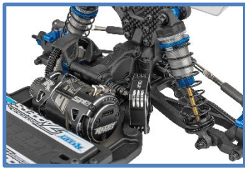
3-Gear Laydown Transmission that maintains original B7 motor position while reducing rotational weight and drag
