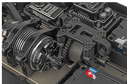
High-volume center differential
