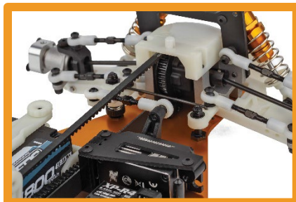
Floating Servo Mount
