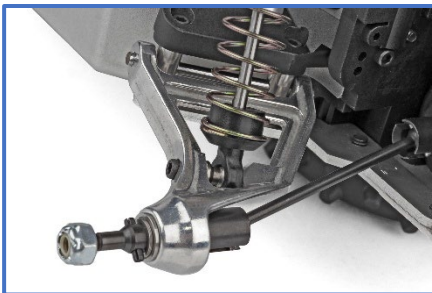
Forged aluminum rear arm and CNC arm mount
