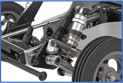
NEW CNC front arm mounts and upper link mounts
