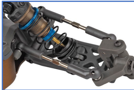
Exclusive grey plastics throughout
