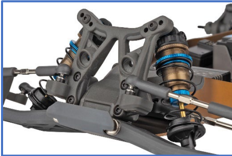
New front and rear molded bulkhead parts
