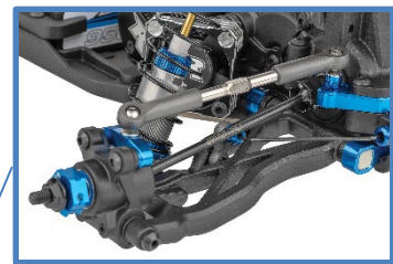
78mm Rear Suspension Arms and 69mm CVA Bones
